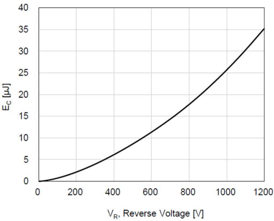
Figure 6. Capacitance Stored Energy
