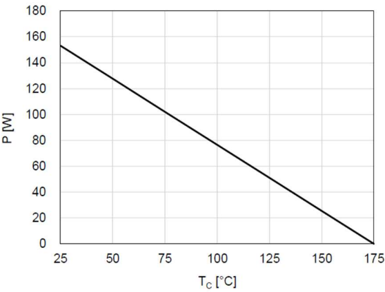
Figure 1. Power Derating
