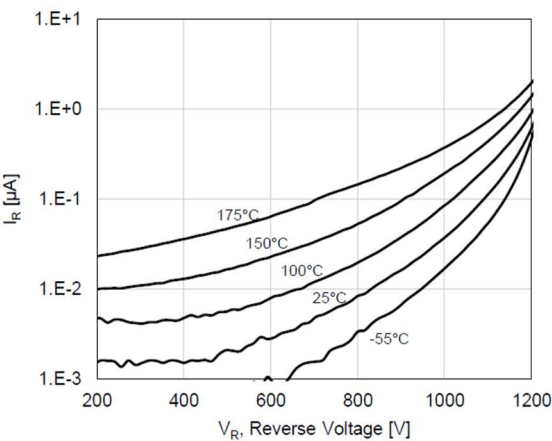
Figure 4. Reverse Characteristics
