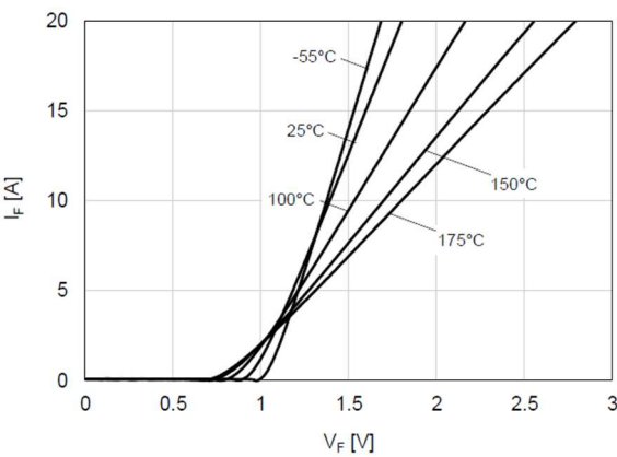
Figure 3 Forward Characteristics
